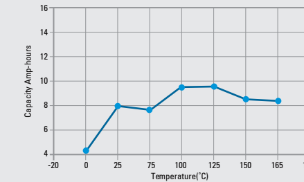
Discharge Temperature vs. Nominal Capacity 16Ω(CC-MR 21) Discharge 0°C to 165°C
