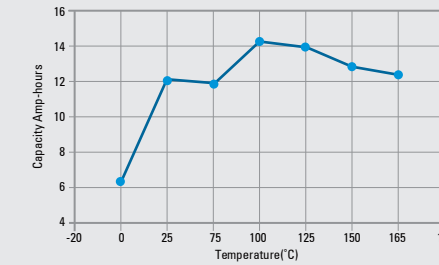
Discharge Temperature vs. Nominal Capacity 14Ω(CC-MR 26) Discharge 0°C to 165°C
